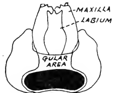
Fig. 235. Ventral aspect of head.
